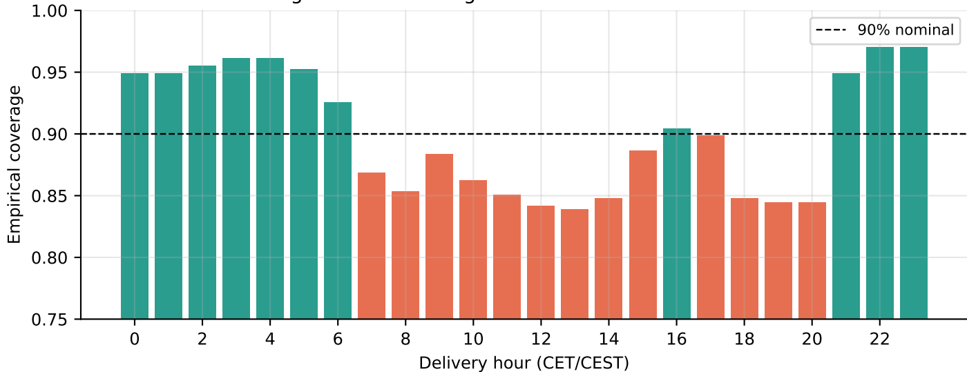
Marginal 90% coverage masks hour-conditional failure
